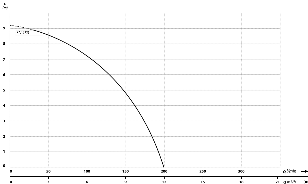
↑ Pumpkurva SN450
