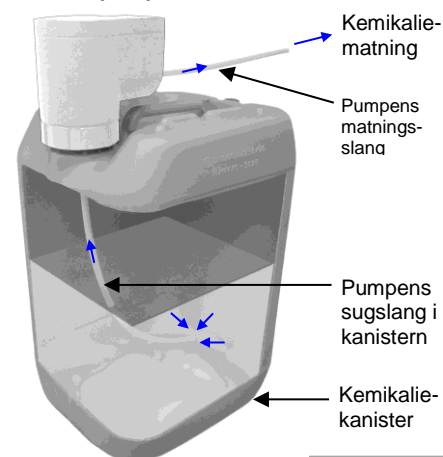
DPT-BC-pump
